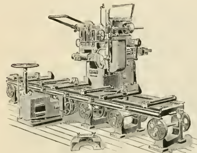
NO. 3 EXTRA LARGE AUTOMATIC CAR GAINING MACHINE.
